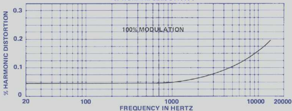
HARMONIC DISTORTION (STEREO AND MONO) AT NORMAL SELECTIVITY
